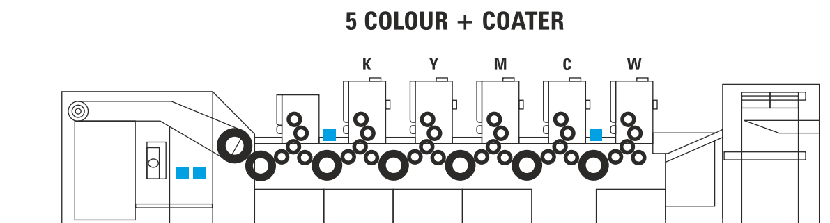
Two ID + Two EOP for Five Colour + Coating Machine
