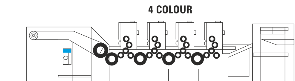
Two UV Interdeck at EOP for Four Colour
