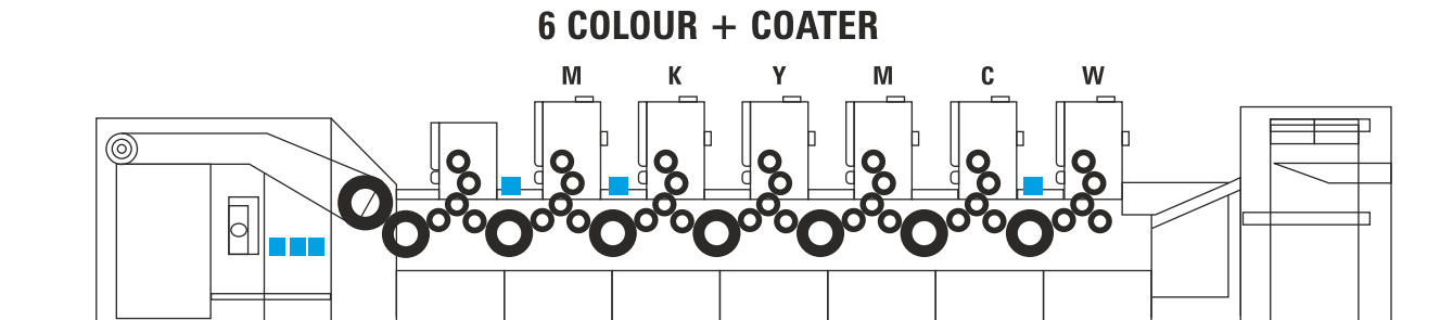
Three ID + Three EOP for Six Colour One Coating Machine
